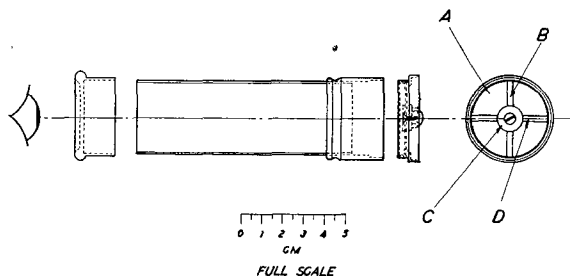
FIG. 2. Diagram of construction of a simple fluoroscope. (A) Fluorescent material (Dupont-Patterson Screen B). (B) Aluminum foil strip. (C) Button with radium-paint. (D) Copper foil strip.
