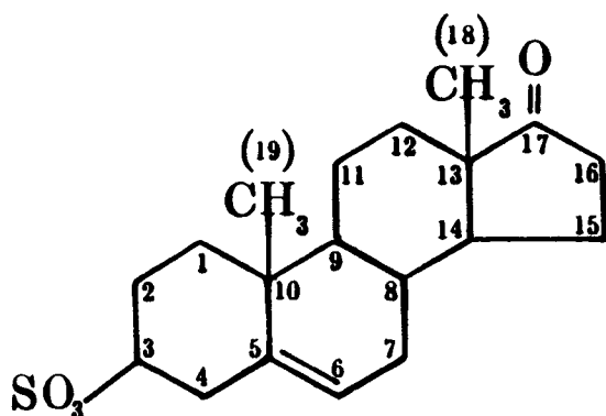
Figure 7. Molecular structure of the C 19 adrenal androgen DHEAS.
