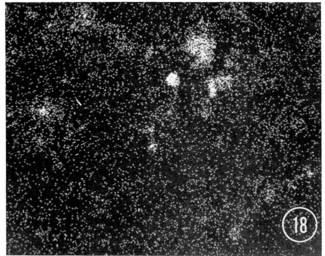
Fig. 18. Case 2. X-ray dot map corresponding to Figure 17. Particles containing silicon produce concentrated clusters of white dots. Particles not containing silicon should be analyzed separately using energy dispersive x-ray analysis.
