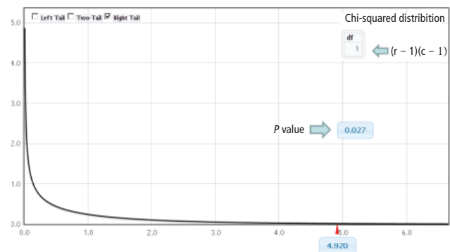
FIGURE 3. Chi-square distribution with 1 degree of freedom. Area under the curve at the test statistic of 4.92 and values more extreme equals the P value of .027.
