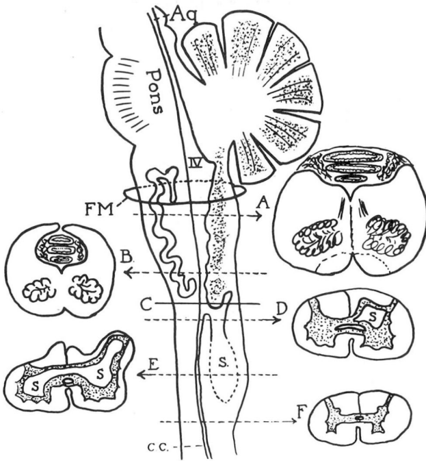
Fig. 3. Schematic drawing of a midsagittal section through the hindbrain and upper cervical cord of an infant with hydrocephalus, Arnold-Chiari malformation, and myelomeningocele. FM indicates the foramen magnum, S the syrinx, c.c. the central canal, and C the level of transection at necropsy. Note the absence of the foramen of Magendie. (Courtesy of Lichtenstein, B. W.: Arch. Neurol. & Psychiat. 49: 881-894, June 1943; A.M.A. Arch. Neurol. & Psychiat.)
