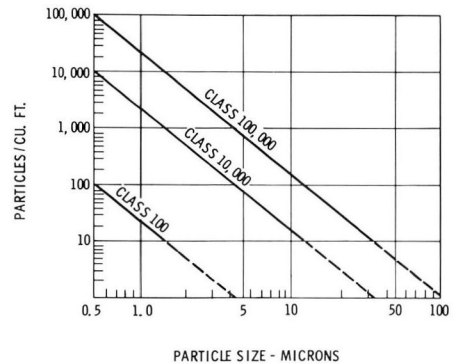
Fig. 2. Each cubic foot of filtered air contains not more than 100 particles 0.5 microns in diameter.
