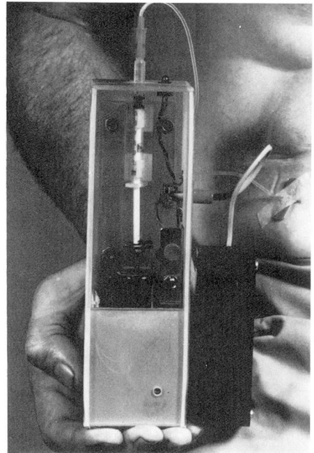
Figure. Portable open loop battery-operated infusion pump.
