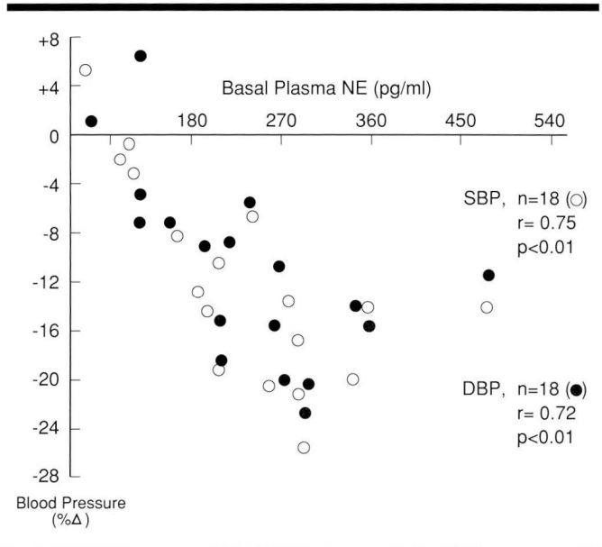
FIGURE 9. Relationship between the circulating levels of norepinephrine (NE) and the arterial pressure response to a centrally acting \alpha_2 -agonist (clonidine). The higher the basal plasma NE, the greater the depressor response to the
