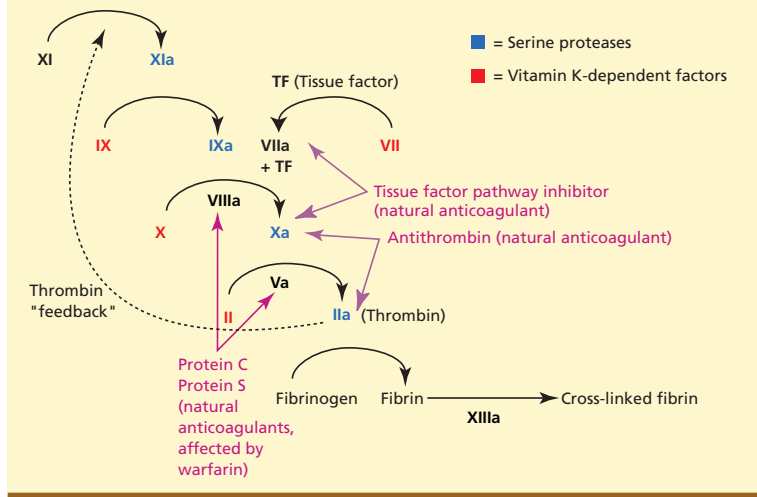
FIGURE 1. Contemporary coagulation cascade with inhibitors (natural anticoagulants).
